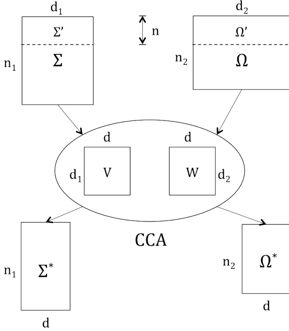
Figure 1: Cross-lingual word vector projection using CCA.
